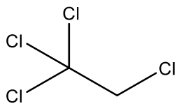
1,1,1,2-tetrachloroethane
