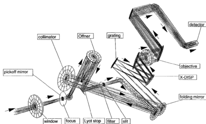
Figure 2 – Infrared spectrometer (working principle)
