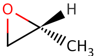
(R)-1,2-epoxypropane
