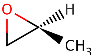
(S)-1,2-epoxypropane
